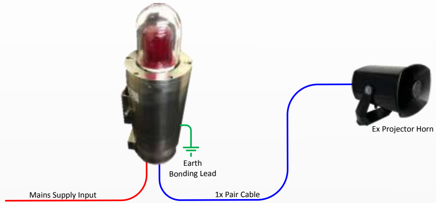
Explosion Proof ZAB1 Beacon fitted with 'S' Option
