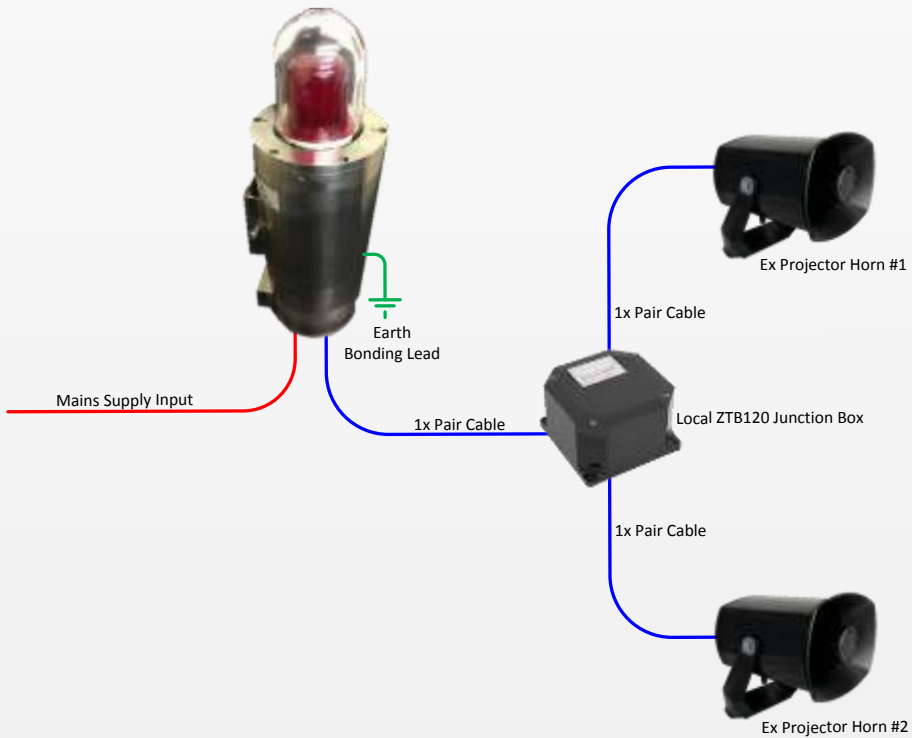
Explosion Proof ZAB1 Beacon fitted with 'S' Option
